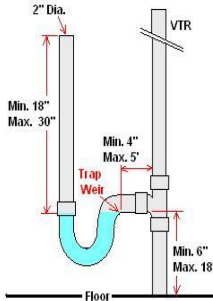
LAUNDRY STANDPIPE Uniform Plumbing Code- UPC
